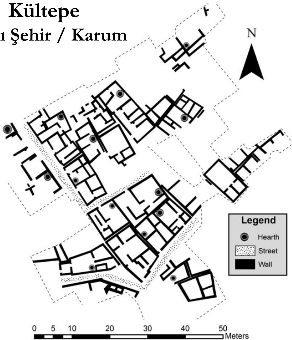
Figure 6.5 Plan of part of a neighborhood in the Karum Kanesh Level II (after T. Özgüç 1986: plan 1)
