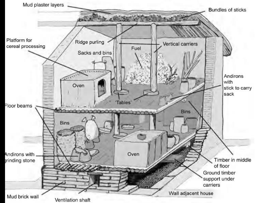
Exterior and interior view of a mud brick house of Ilıpınar VI (after Coockson 2008)
